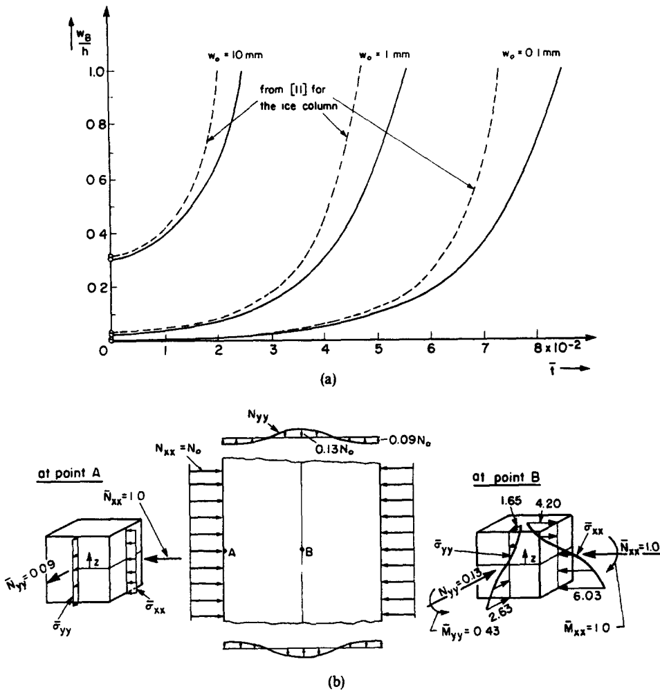
Fig. 5. Viscous behaviour of imperfect ice plate undergoing cylindrical bending. (a) Time-deflection behaviour. (b) Stress resultant and stress distribution for t = 0.056 ( w_0 = 1 \text{ mm} , w_B = h ).
